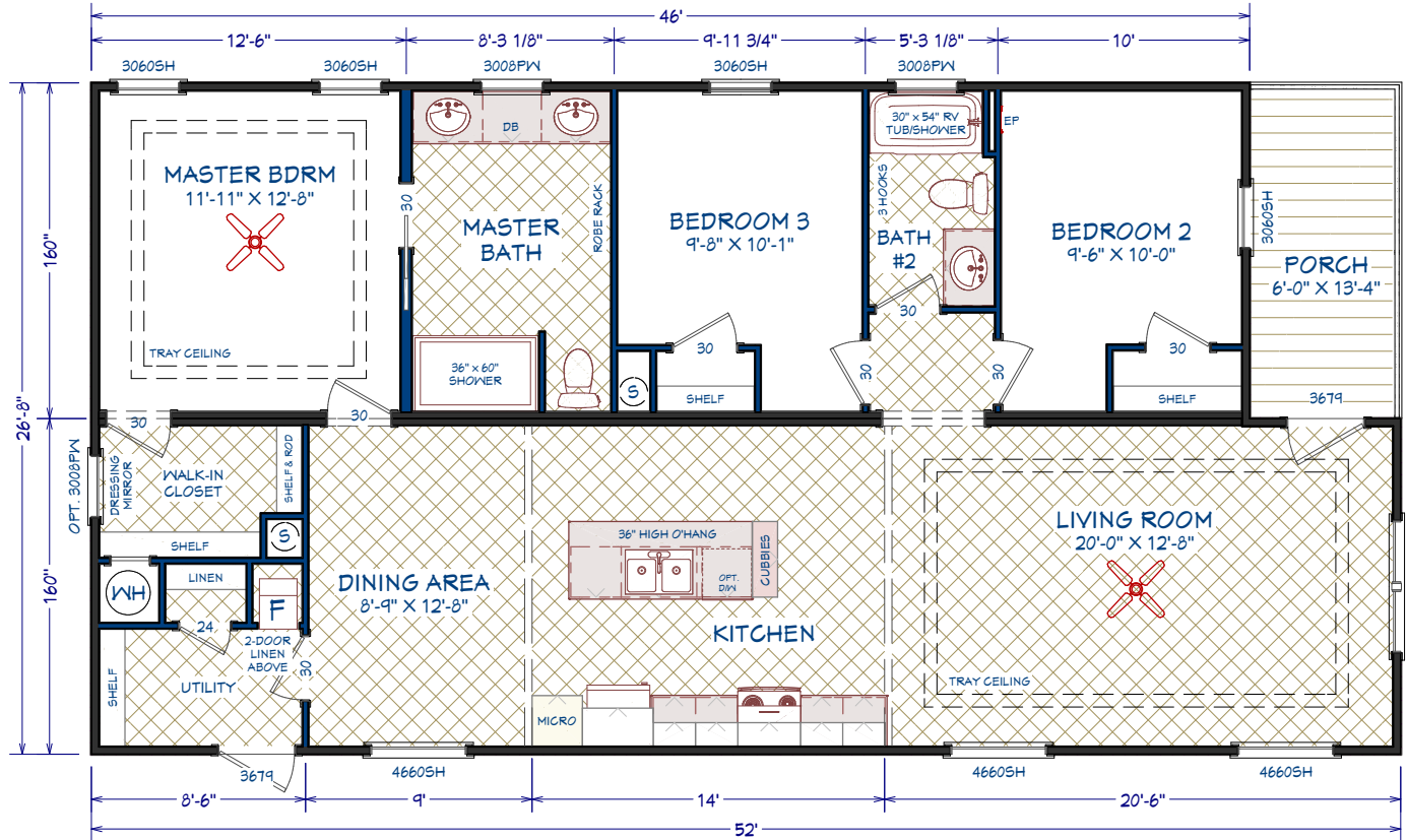
LIVING AREA 1307 SQ FT
